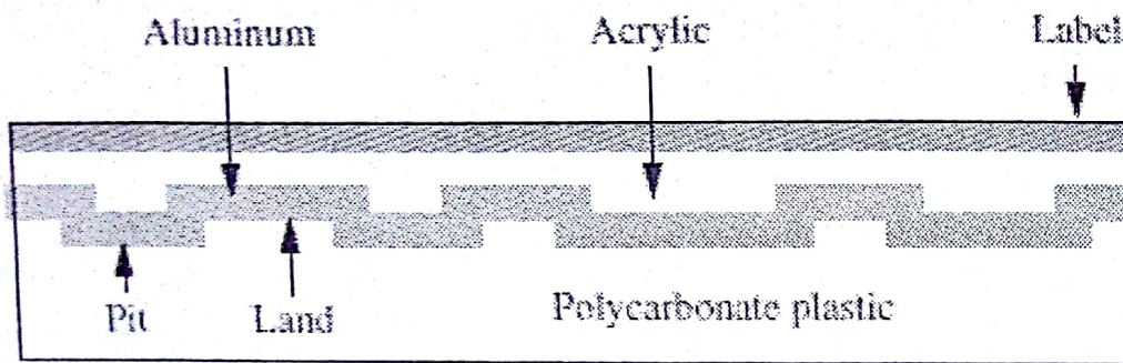
(a) Cross-section
