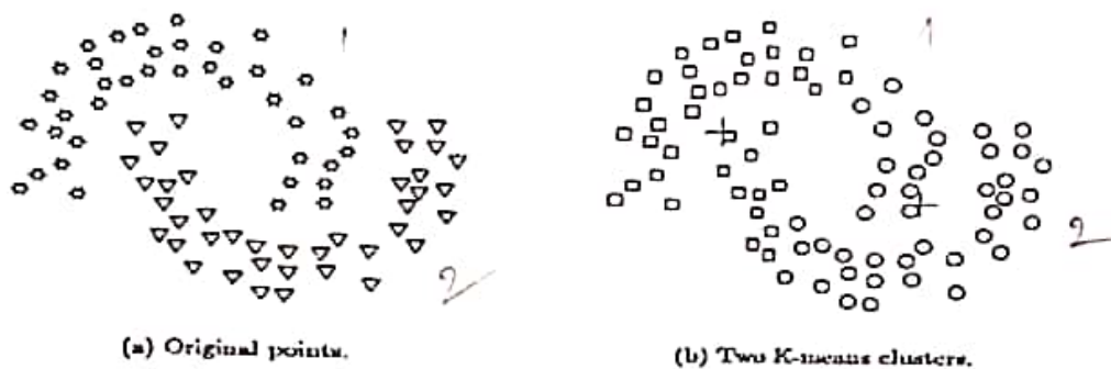
Figure 8.11. K-means with non-globular clusters.
