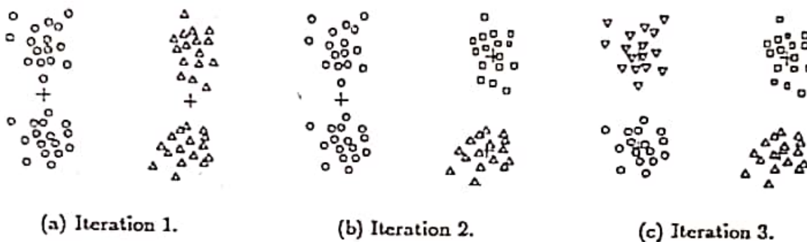
Figure 8.8. Bisecting K-means on the four clusters example.
