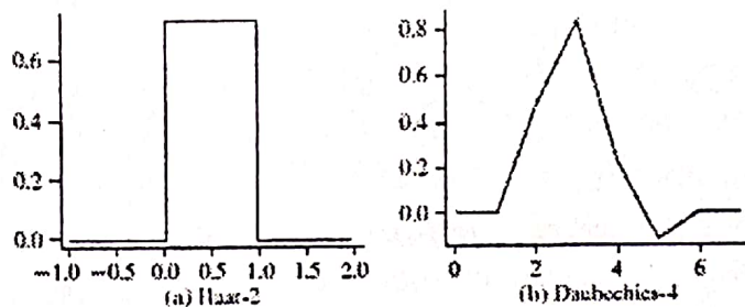
Examples of wavelet families. The number next to a wavelet name is the number of vanishing moments of the wavelet. This is a set of mathematical relationships that the coefficients must satisfy and is related to the number of coefficients.
