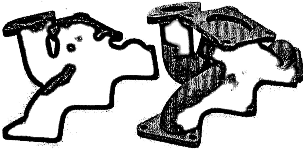
Figure 7.6: Cast metal (left) and RP pattern for sand casting (Courtesy of Helysis Inc.)
