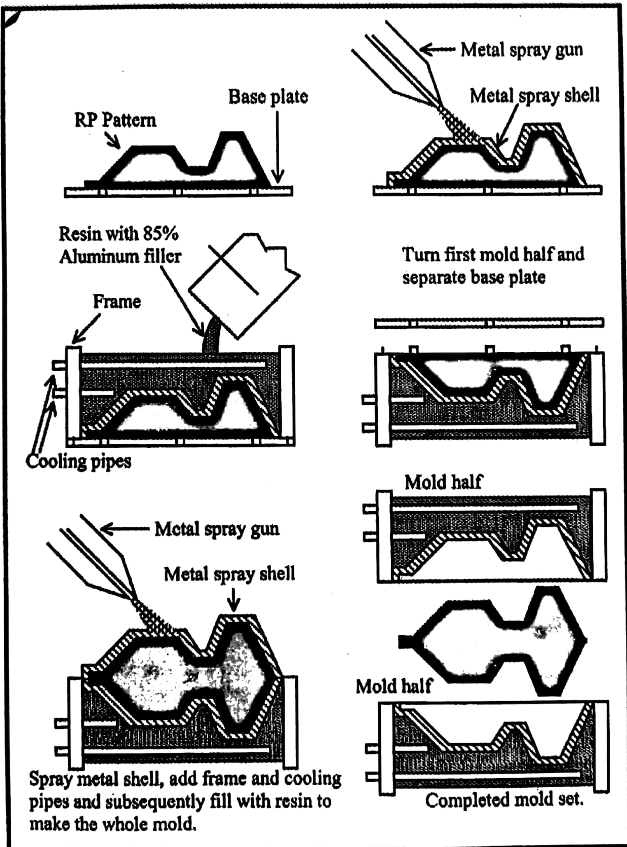
Figure 7.4: A metal arc spray system
