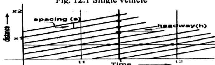
Fig. 12.1 Single vehicle
