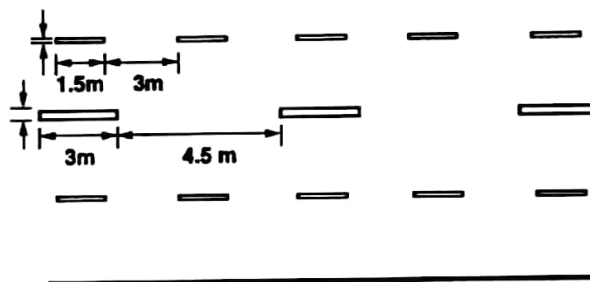
Centre line and lane marking for a four lane road
