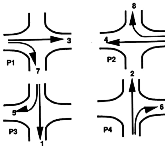
Fig.19.2 One way of providing four phase signals
