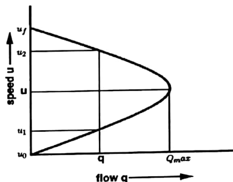
Fig. Speed-flow diagram
