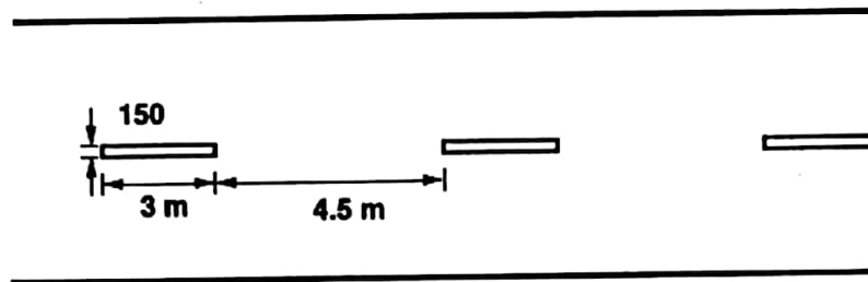
Fig. Centre line marking for a two lane road
