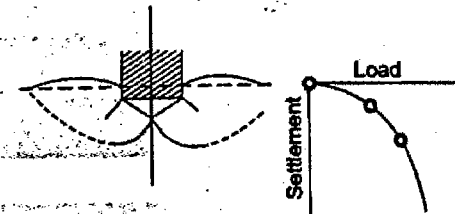
Fig. 15.3 Local shear failure
