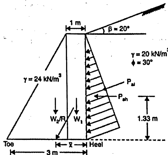
Fig. 13.72 Retaining wall (Ex. 13.27)
