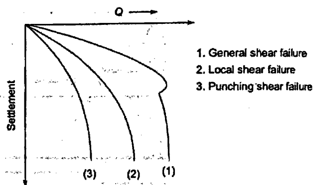
Fig. 15.5 Load-settlement curve for soils
