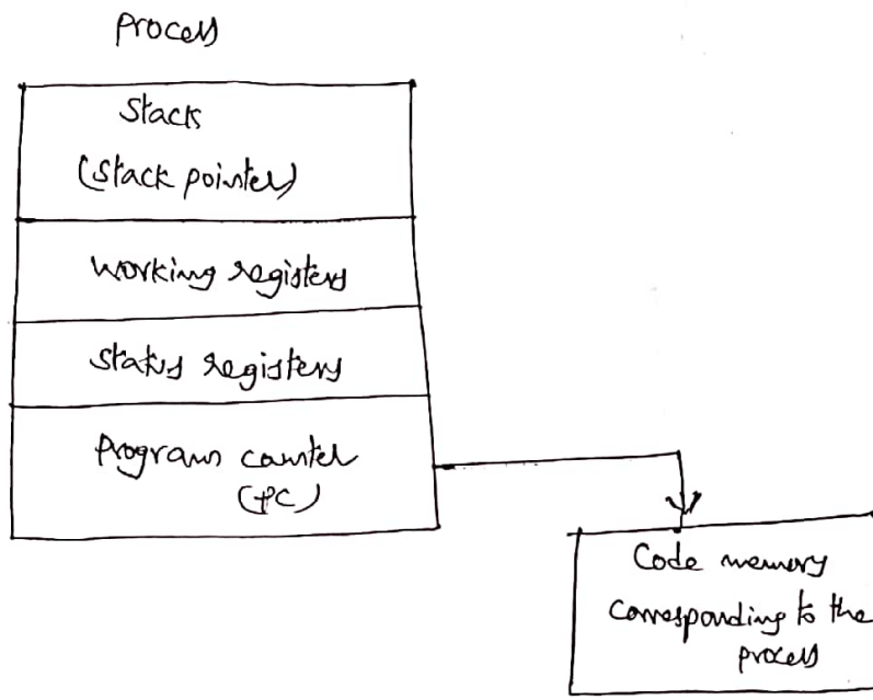
Fig:- structure of a process
