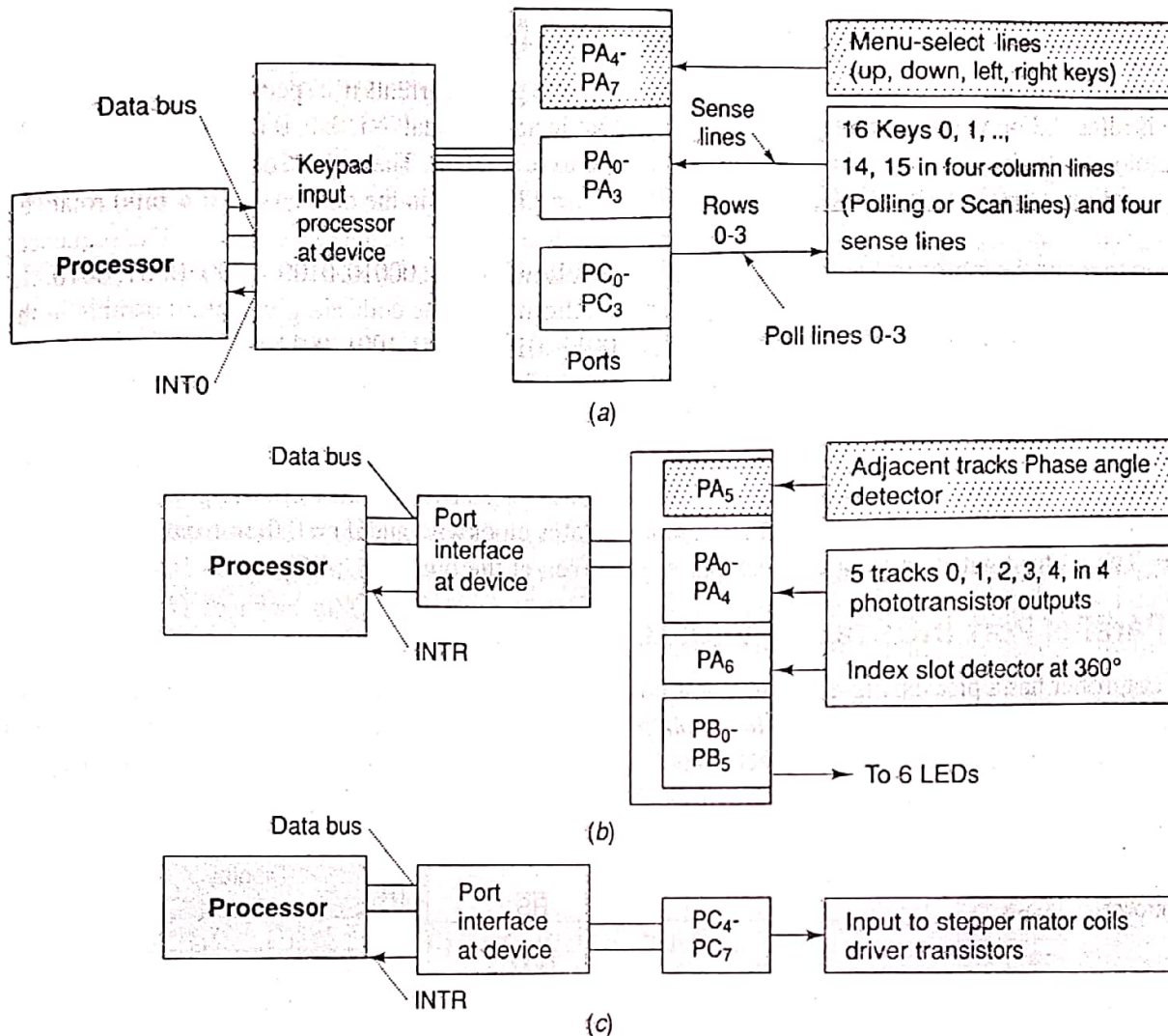
Fig. 3.5 (a) Parallel input port A and a four bit output port C used for interfacing a set of 16 keys in keypad and four menu select keys (b) Parallel input port A connected to an encoder circuit which senses the rotated or linear position of a moving shaft and port B connected to 6 LEDs (c) Four bit parallel output port C connected to a stepper motor
