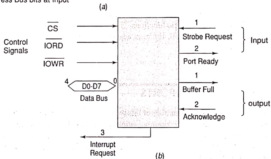
Fig. 3.4 (a) Parallel input port, output port, and a bi-directional port for connecting the device (b) The handshaking signals when used by the IO ports
