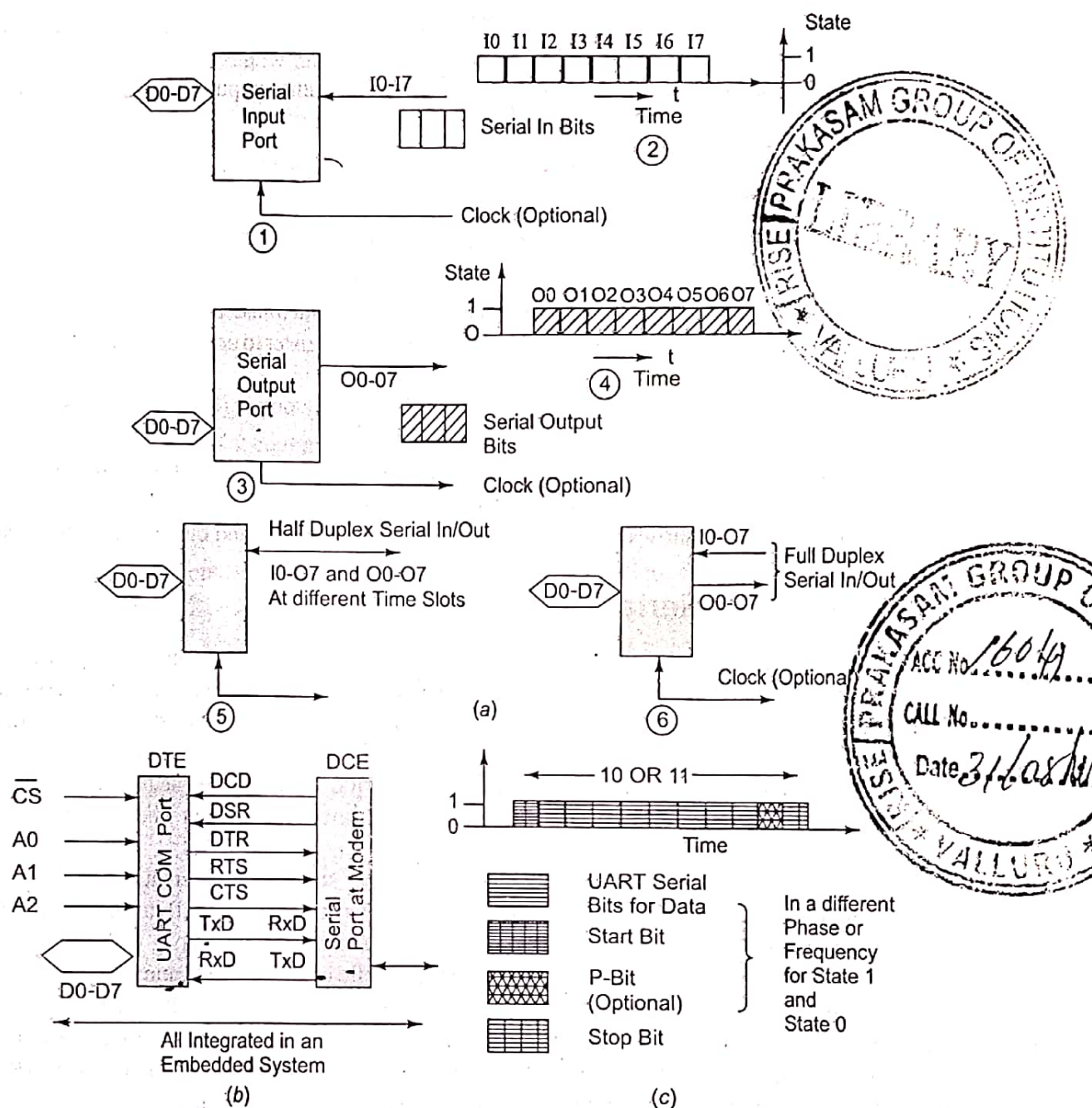
Fig. 3.1 (a) Input serial port, Output Serial port, Bi-directional half-duplex serial port, and Bi-directional full-duplex serial port (b) Handshaking signals at COM port in computer and (c) a UART serial port bits
