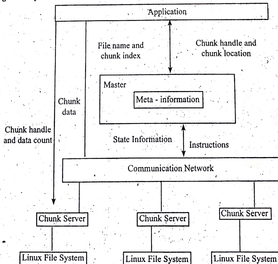
Figure: GFS Cluster
