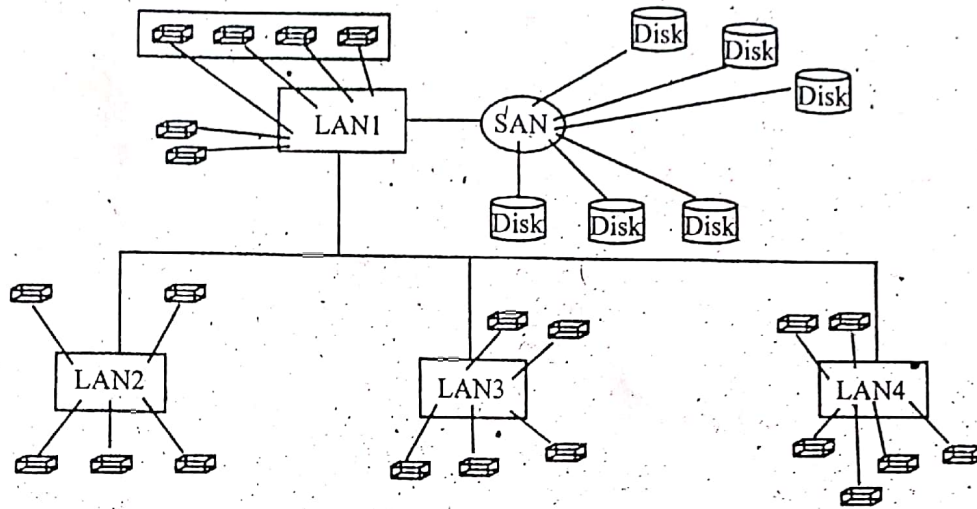
Figure: GPFS Configuration
