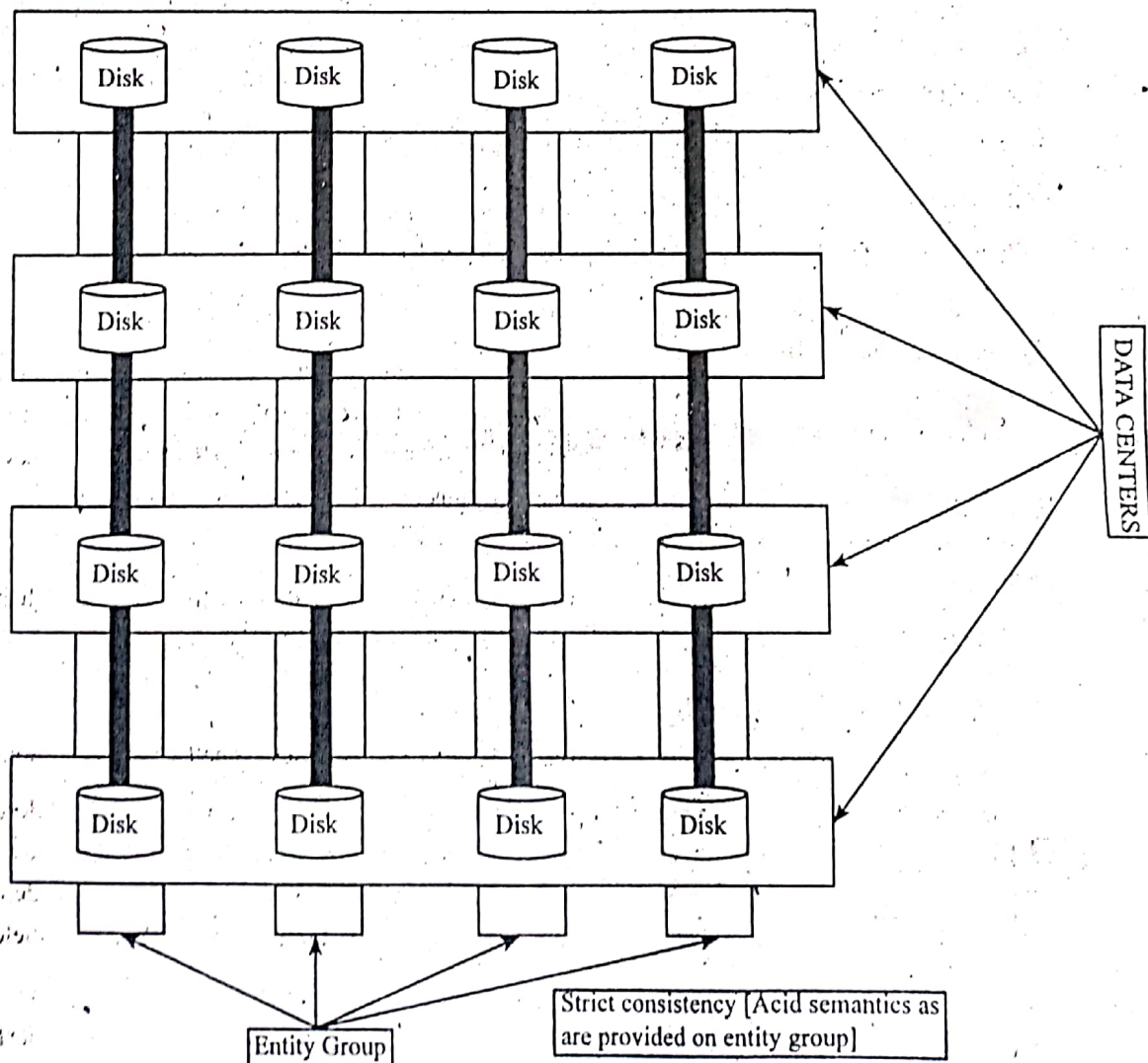
Figure: Megastore Organization
