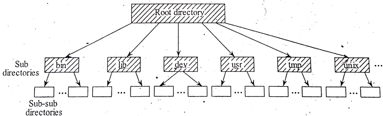
Figure: Unix Directory/File Structure (A Snapshot of Upside Down Tree)
